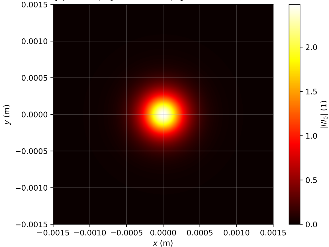
Intensity profile I(x, y, z = 2.707m)/I_0 , P_{in}=1.0P_{cr} , artificial time
